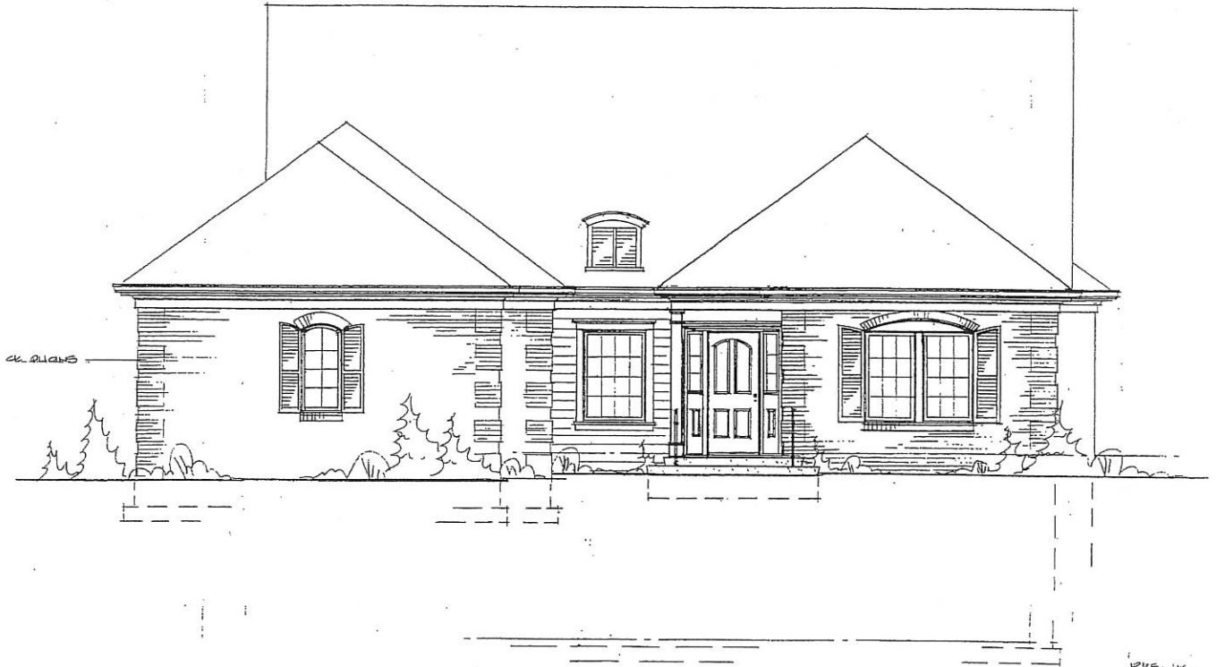
PROPOSED FRONT ELEVATION 1/4" = 1'-0"
