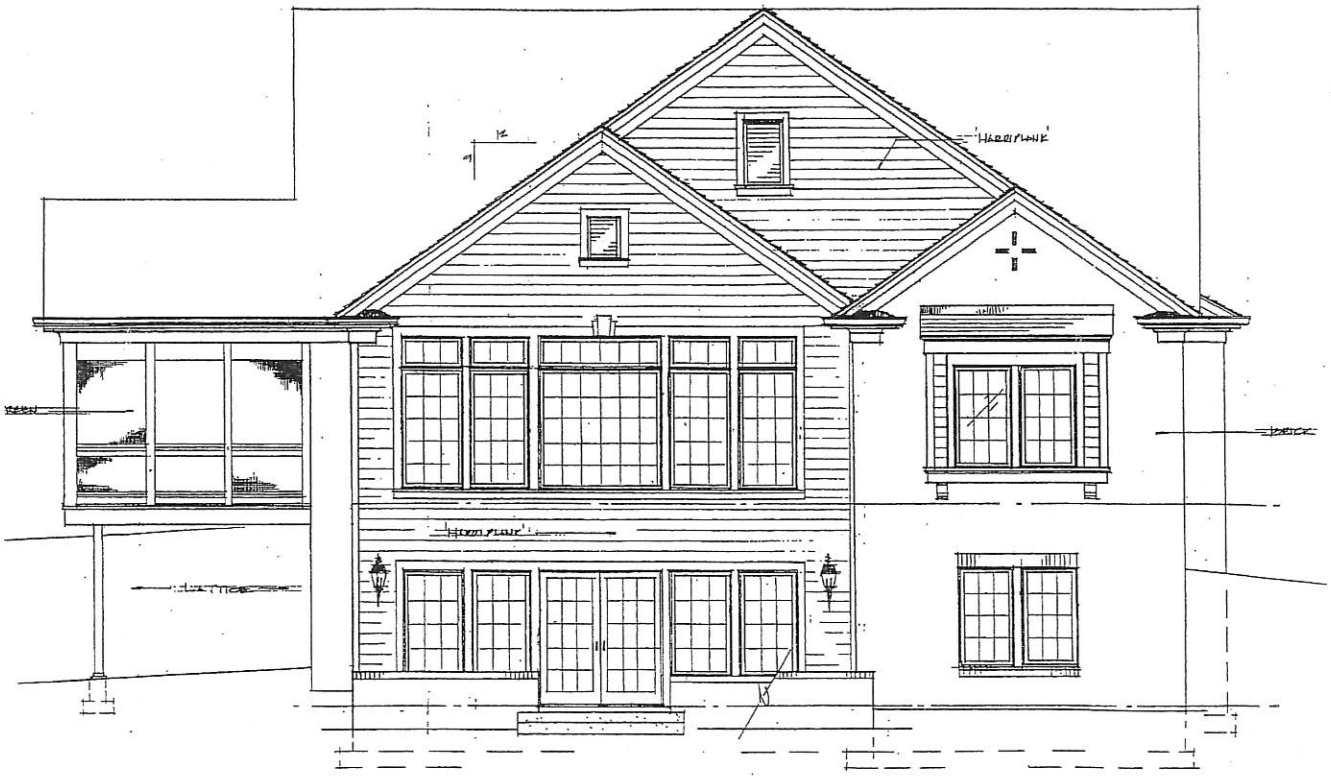
LAKE VIEW ELEVATION 1/4" = 1'-0"
